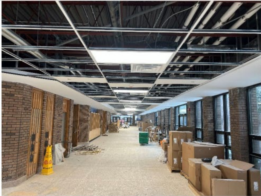
Ceiling grid installed at first floor entrance corridor
